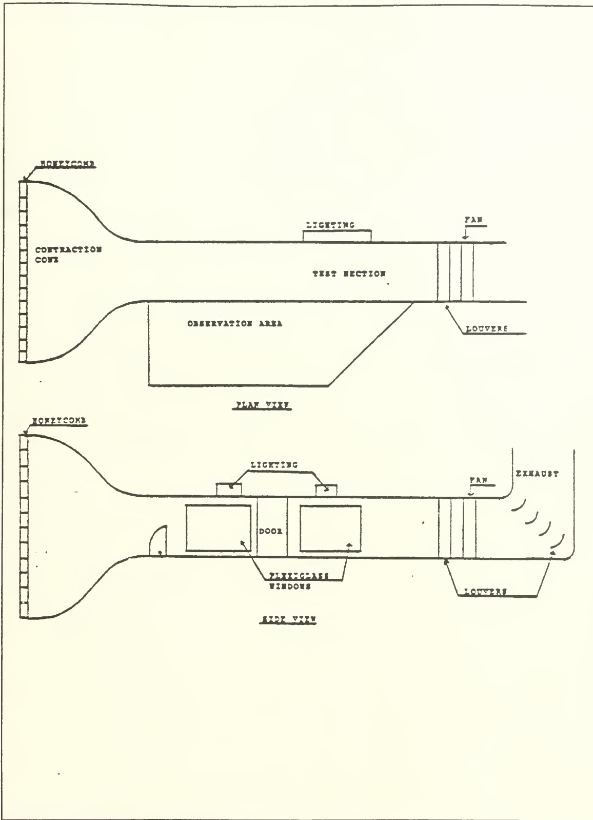
Figure 5.2 Tunnel Layout
